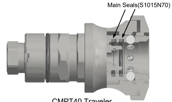
CMPT40 Traveler. Section view to show seals.
