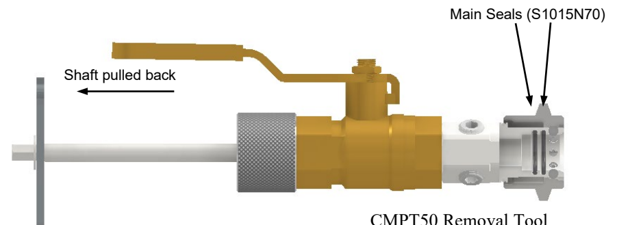
CMPT50 Removal Tool Section view showing tool seals
