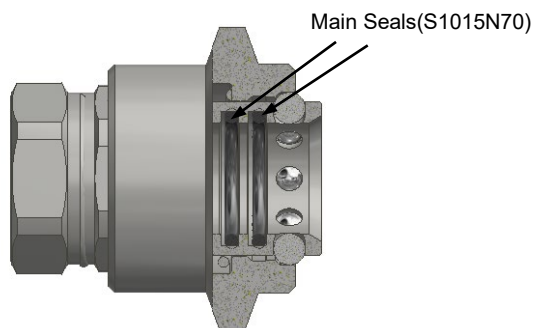
CMPT10 MBE Connector. Section view to show seals.
